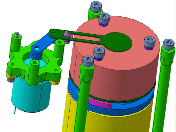
UV photometer
