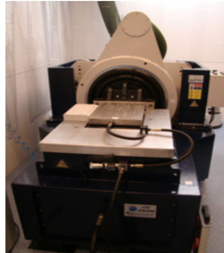
Mechanical tests (random) with CNRS-LATMOS facilities
